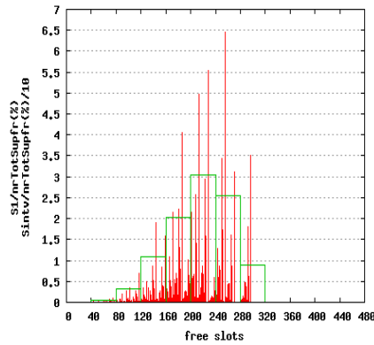
Fig. 7. Free slots for op. mode 3, P=0.75 .
