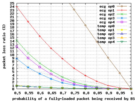
Fig. 2. Packet loss ratio for ECG and T traffic.
