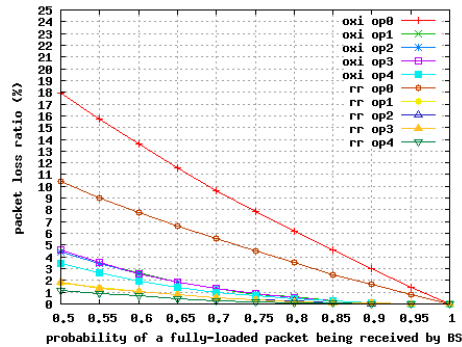
Fig. 4. Packet loss ratio for OXI and RR traffic.
