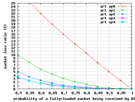
Fig. 3. Packet loss ratio for ART traffic.
