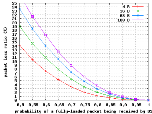
Fig. 1. ECG packet loss ratio for several beacon payloads.
