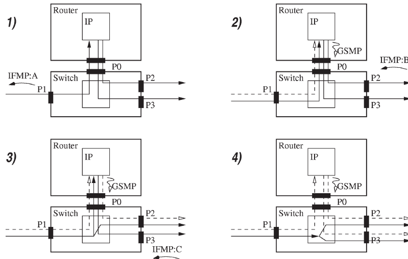
Figure 1. IPswitching multicast cut-through.
