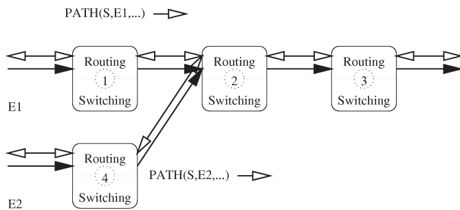
Figure 10. Initial routing path with aggregation.
