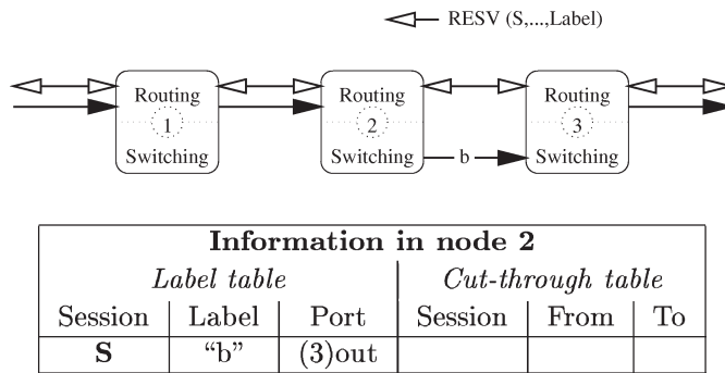
Figure 4. Starting of labeling.
