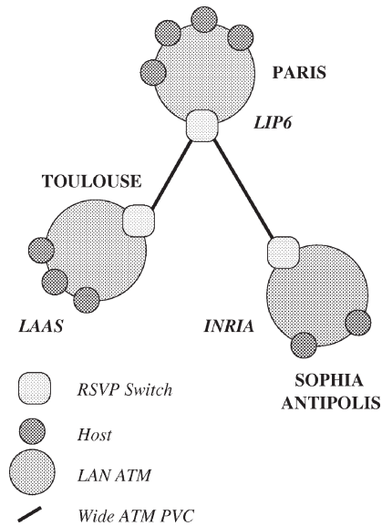
Figure 15. MIRIHADÉ testbed.
