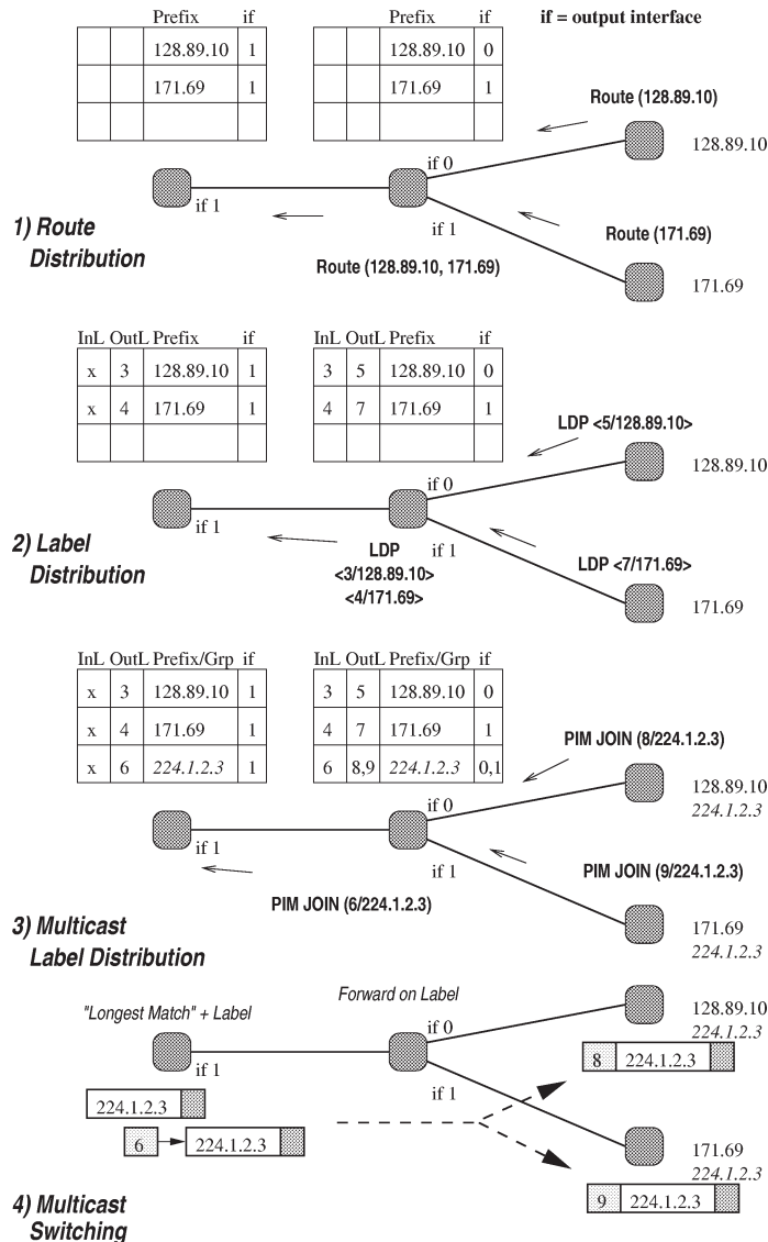
Figure 2. Creating an MPLS multicast.
