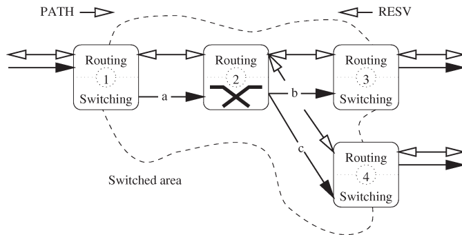
Figure 5. Enabling unicast cut-through.
