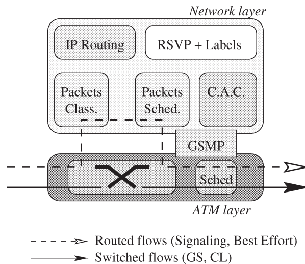
Figure 14. RSVP Switch architecture.
