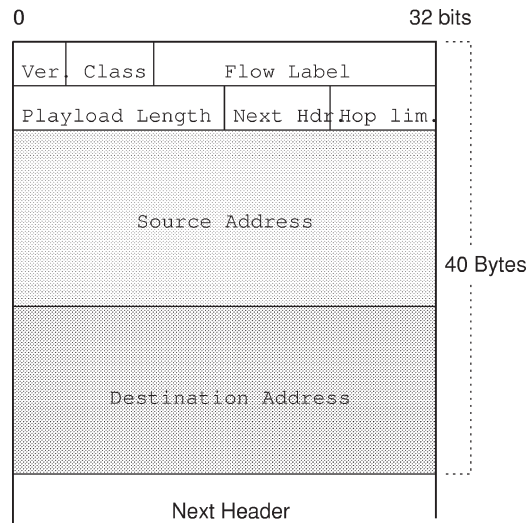
Figure 13. Ipv6 header.
